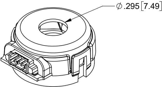
H-OPTION COVER (COVER HOLE FOR SHAFT LENGTHS OVER .395 [10.03])
