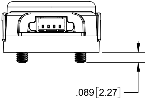
M-OPTION BASE M2.5 X 4 SCREWS (2X INCLUDED)
