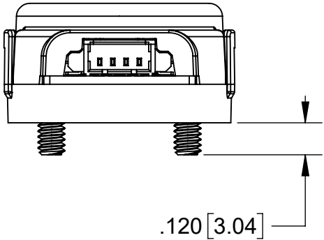
DEFAULT BASE #3-48 X 3/16 SCREWS (2X INCLUDED)
